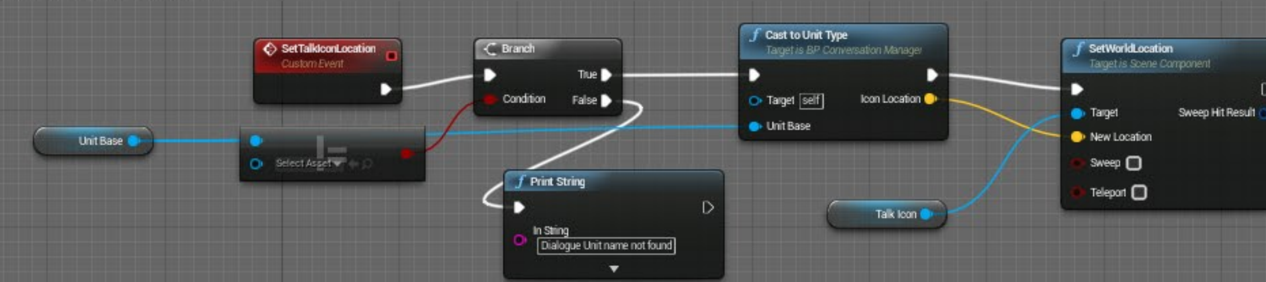
Set world location of icon
